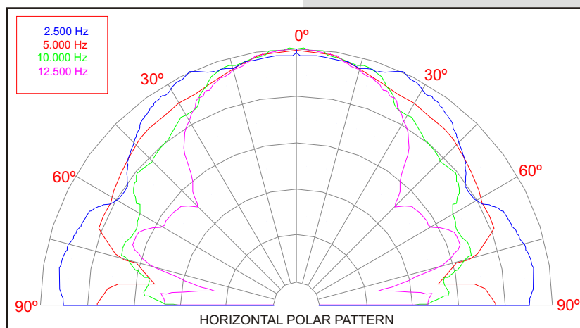
HORIZONTAL POLAR PATTERN
