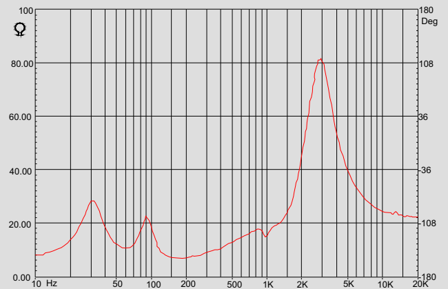
IMPEDANCE CURVE
